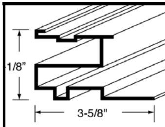
Inwall # 2 without Liner Bead #1041P
