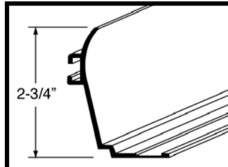
Reuseable Deck Form Extrusion #1308P
