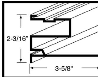
Inwall # 3 Vinyl With Liner Bead #1042P
