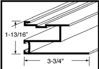
Inwall # 5 for Fiber Optics #1302P
