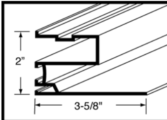
Inwall # 6 for Fiber Optics # 1303P Vinyl Liner
