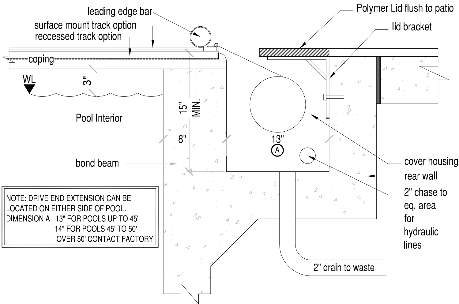
STEP DECK DETAIL
