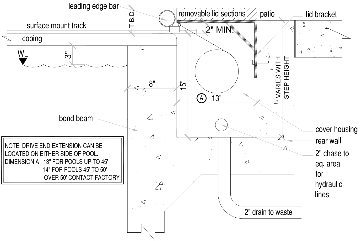
STEP DECK DETAIL
