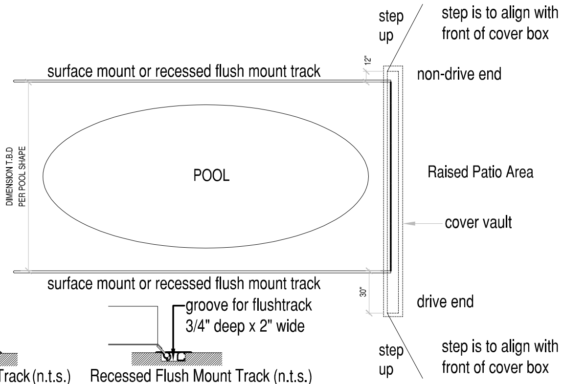
STEP DECK DETAIL
