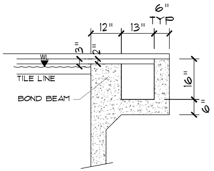
SECTION VIEW
